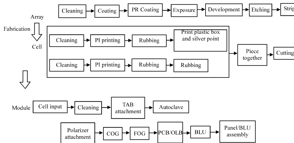
Fig. 1: LCD panel manufacturing process; COG: Chip on Glass; FOG: Film on Glass; PCB: Printed Circuit Board; OLB: Outer Lead Bonding and BLU: Back Light Unit
