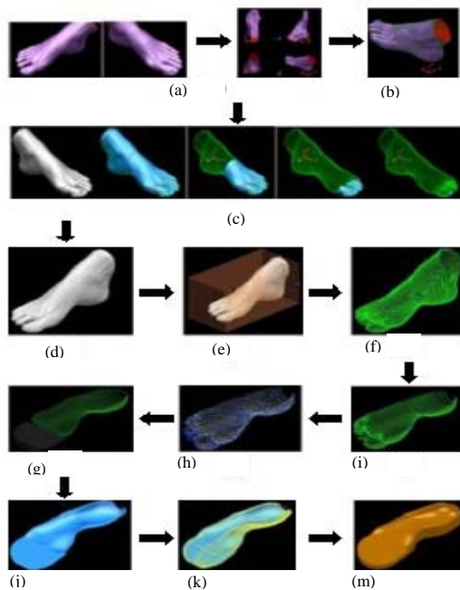
Fig. 8: CBS-modeling iso_diabetes involved in PowerShape 2016: a) Mesh importing and pre processes; b) Rewiring; c) Repoint, built and verification 3D surface to solid foot with solid doctor; d) 3D solid model foot from mesh; e) Oblique processing; f) Foot wireframe; g) Wire support; h) Repoint wireframe curve; i) Wire reconstruction; j) Surface generating; k) Surface curve editing and l) 3D solid iso_diabetes
