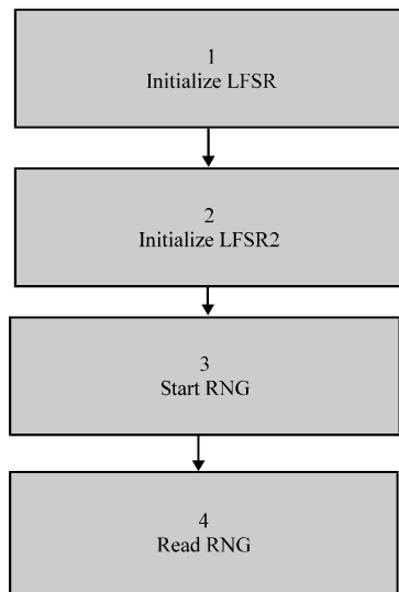
Fig. 3: RNG flow
