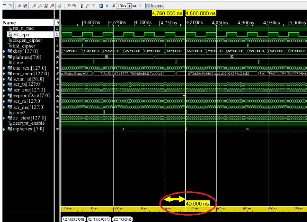
Fig. 8: The total ciphering time is a single CPU clock cycle, i.e., 40 nsec
