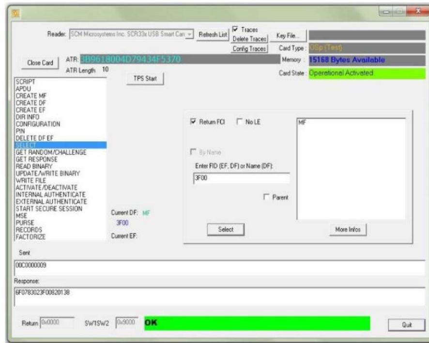
Fig. 12: Real-time testing with a reader of the ATR reading, SELECT MF and GET RESPONSE commands
