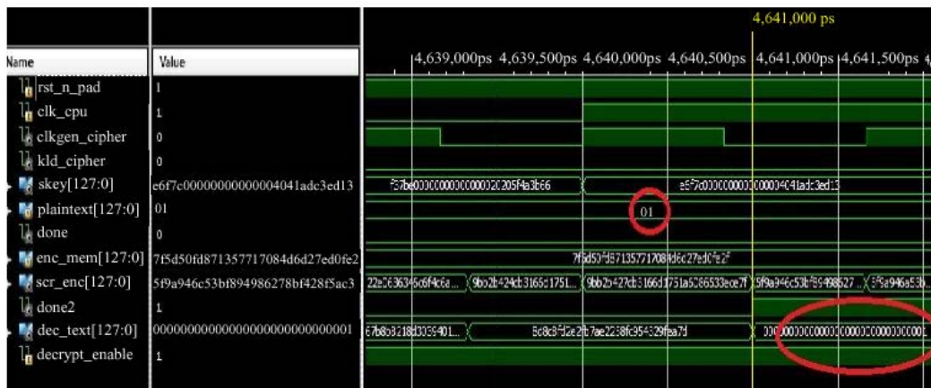
Fig. 9: Secured data is successfully decrypted to its plaintext value i.e. Hex 01
