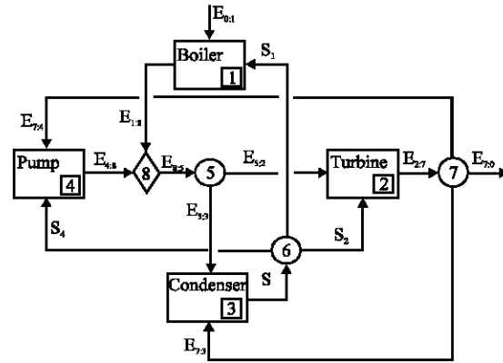
Fig. 3: Productive structure of the power plant for the exergy-negentropy method
