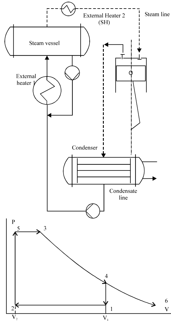
Fig. 2: a) Schematic of the steam engine, condenser and steam vessel and b) Diagram of the compression and expansion of the reciprocated steam engine model
