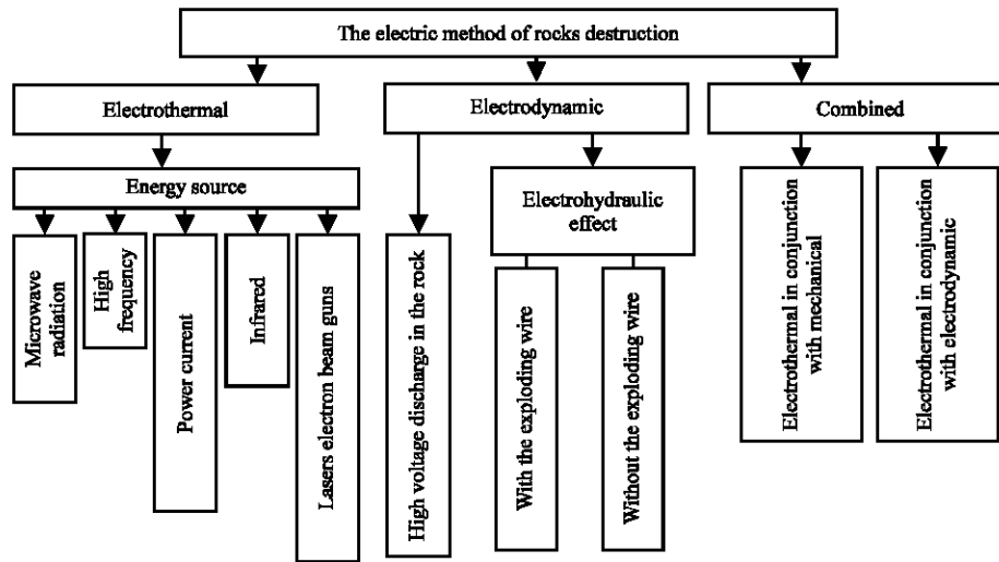
Fig. 5: Classification of electrical methods of destruction of rocks
