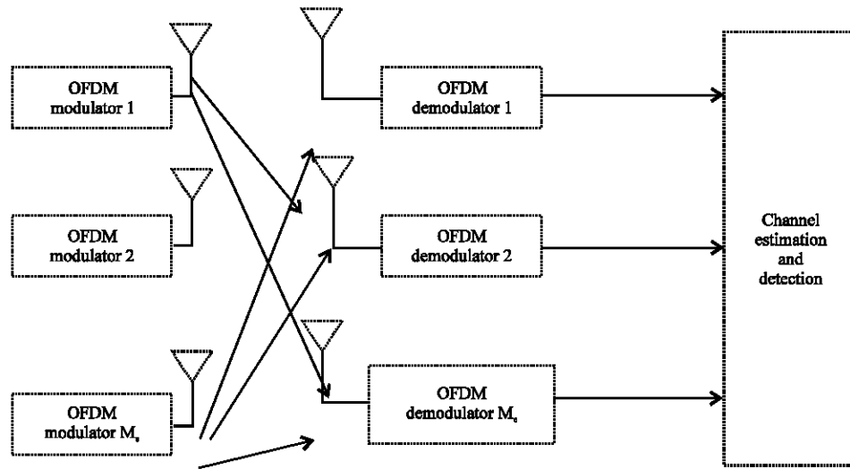
Fig. 2: CDMA/MIMO receiver
