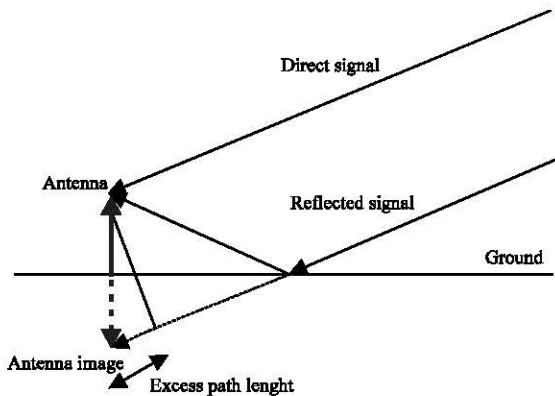
Fig. 2: Multipath phenomenon
