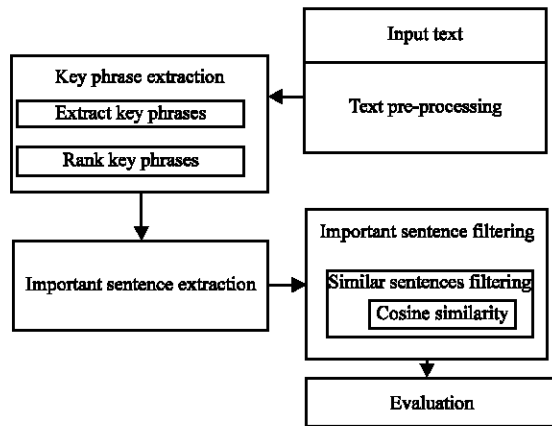
Fig. 1: Overall structure of Arabic text summarization
