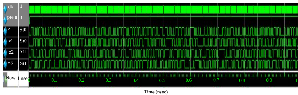
Fig. 6: Multi-channel PingPong 256 results from gate level test
