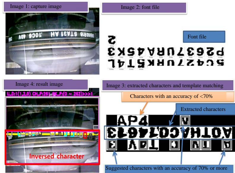
Fig. 5: Image processing algorithm implementation
