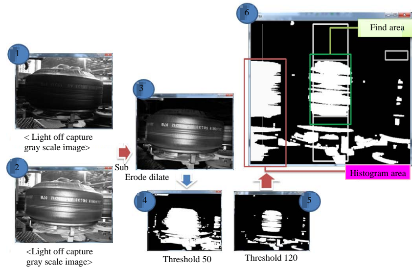
Fig. 6: Preprocessing algorithm for green-case character detection system
