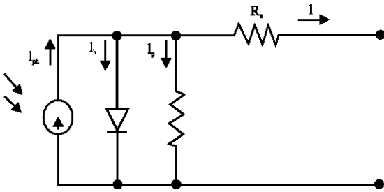
Fig. 2: The equivalent circuit of a solar cell
