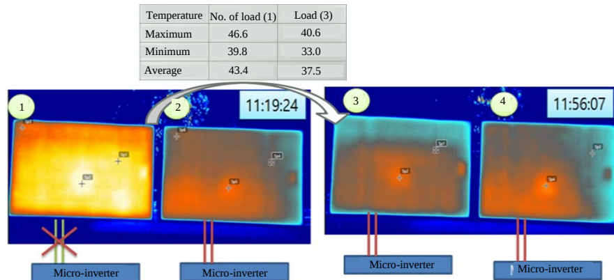
Fig. 7: Thermal image according to load connecting status
