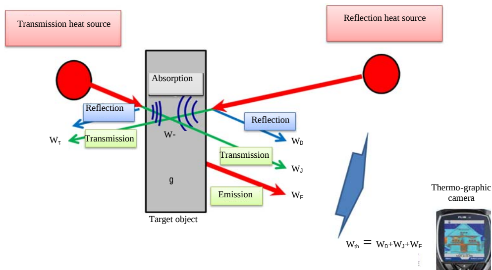
Fig. 4: Principle of thermos-graphic camera
