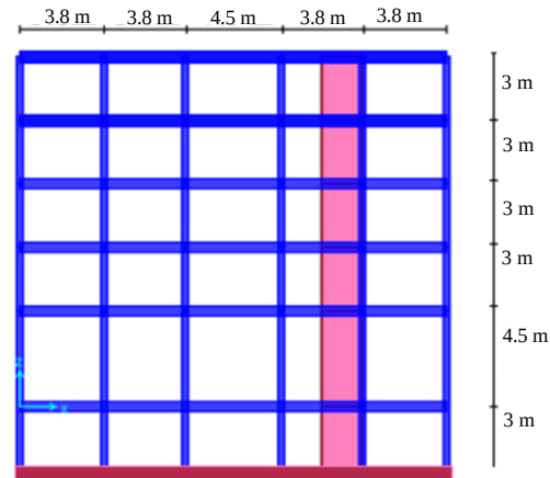
Fig. 3: Building B3-XZ plane (Front elevation)
