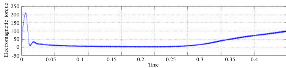
Fig. 15: Electromagnetic torque of PMSM with time when U_1 = constant; Rotor speed by rad/sec with time
