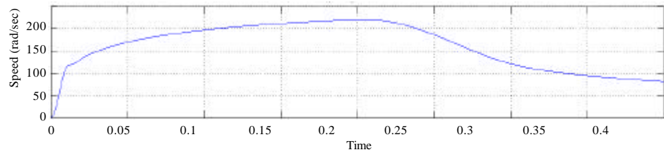
Fig. 14: Speed of PMSM with time when U_1 = Constant; Rotor speed by rad/sec with time
