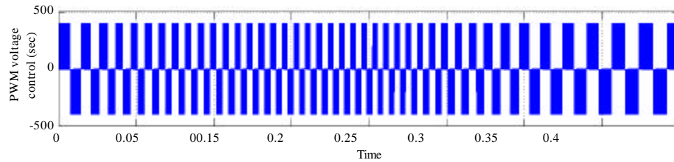
Fig. 16: The line voltage U_{ab} with time when U_1 = Constant
