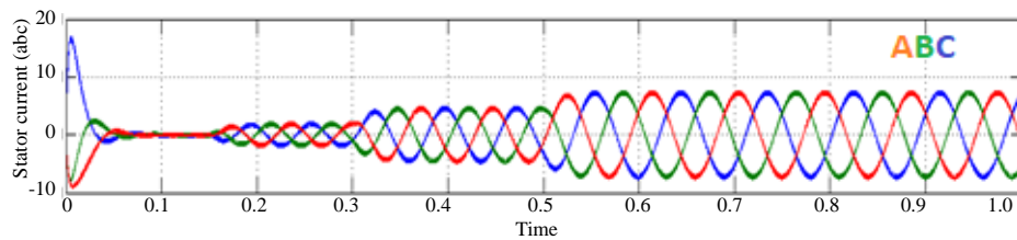
Fig. 4: Three-phase stator current A-C with time when U_1 = 20 V; Three-phase stator current ABC with time
