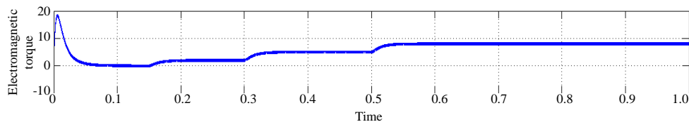
Fig. 6: Electromagnetic torque with time when U_1 = 20 V
