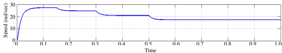
Fig. 5: Speed of PMSM with time when U_1 = 20 V; Rotor speed by rad/sec with time
