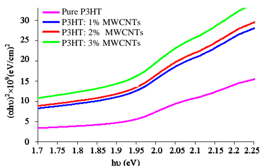
Fig. 12: Relation between (\alpha h\nu)^2 versus photon energy
