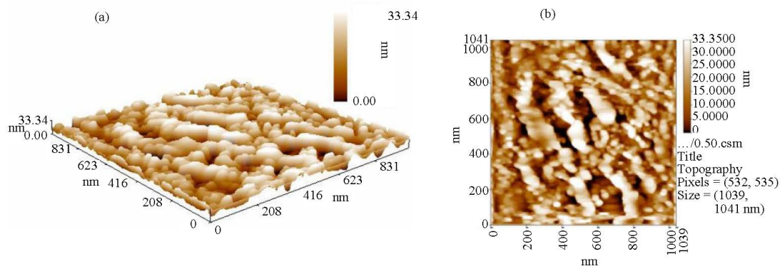
Fig. 5: AFM images of P3HT: 2% MWCNTs for; a) 3-D and b) 2-D
