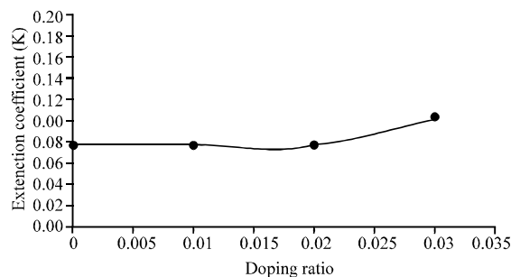
Fig. 15: Extinction coefficients ( k ) as a function of doping ratio
