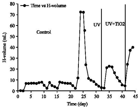
Fig. 5: Hydrogen volume produced along 44 days in TPBR
