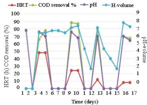
Fig. 4: Relationship between HRT, pH with COD and (H) volume production by mixed culture
