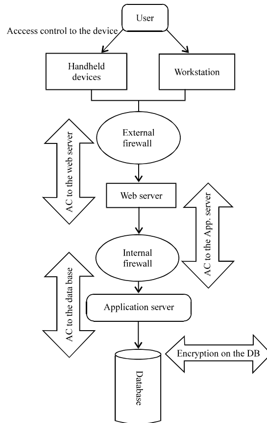
Fig. 6: Data motion
