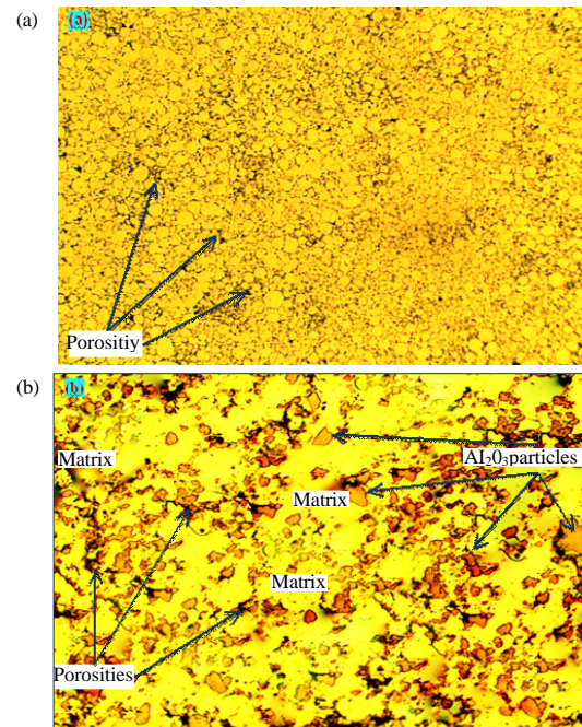
Fig. 2a: Optical Microstructure of Al-Mg-Si matrix alloy (Alloy-1) underwent sintering process (460°C/1.5 h) and b) Optical micrograph of matrix of Al-Mg-Si/Alumina after sintering process
