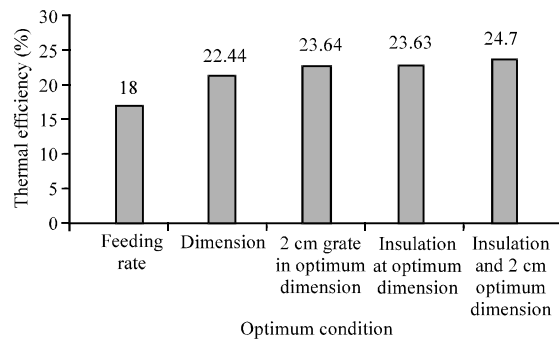
Fig. 13: Thermal efficiency at optimum condition
