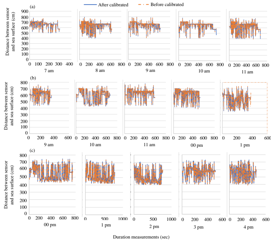
Fig. 6: Sensor reading comparison before and after calibrated from 27-29th September 2016; a) Graph of see waves measurment in 27th September 2016 Sungai Suci Bangkulu; b) Graph of see waves measurment in 28th September 2016 Sungai Suci Bangkulu and c) Graph of see waves measurment in 29th September 2016 Sungai Suci Bangkulu
