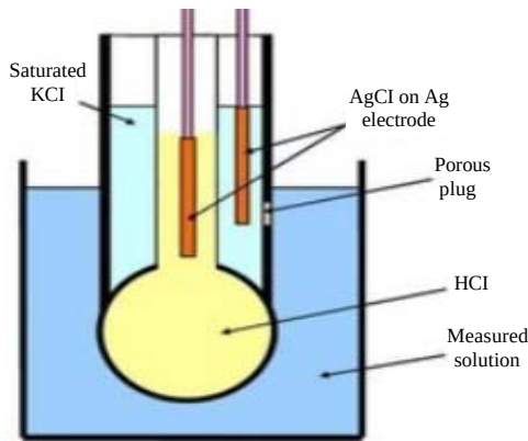
Fig. 2: Structure of pH meter
