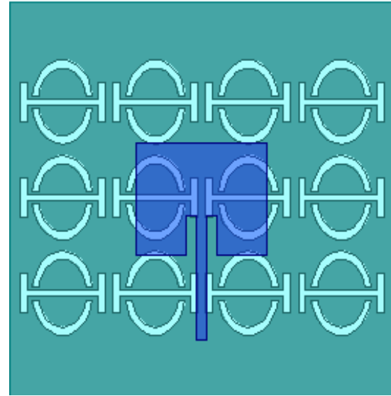
Fig. 3: Square antenna with meta-phi cell printed on ground plane
