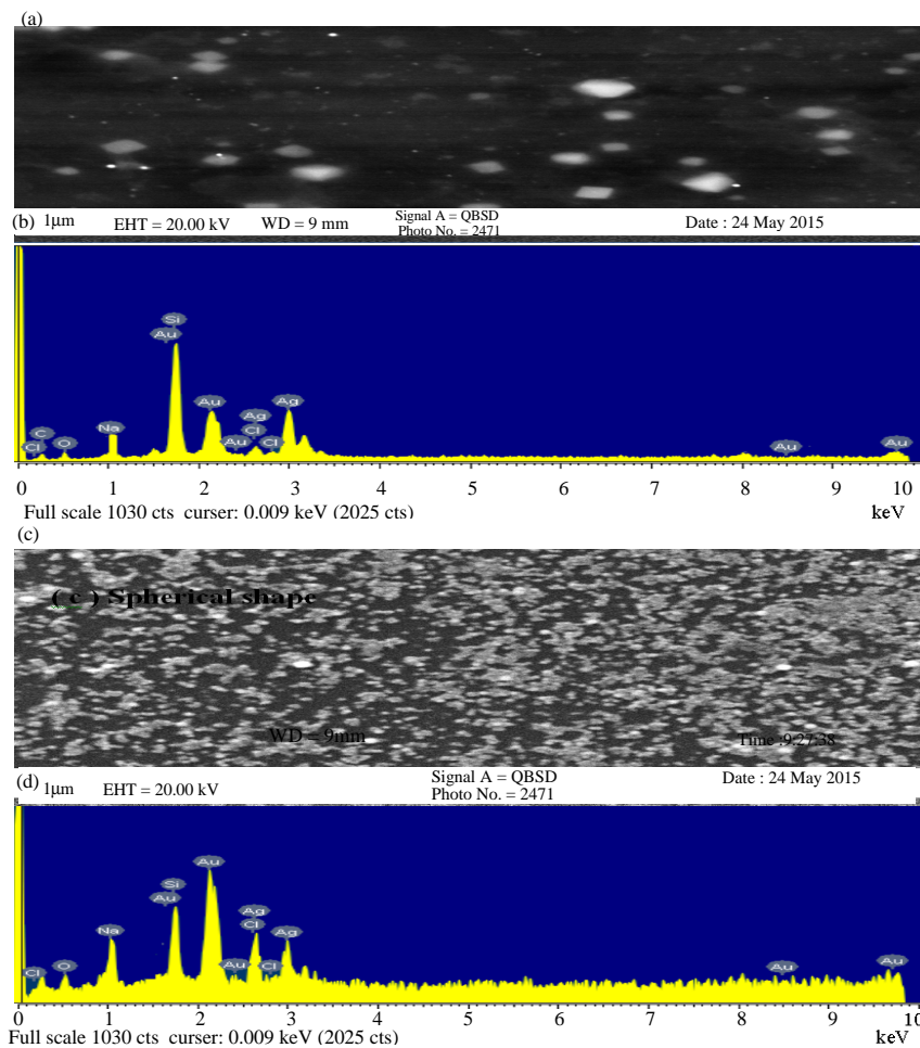
Fig. 6: a) The SEM images and EDX scheme of nanoparticles of \text{Au}_{50}\text{Ag}_{50} alloy colloidal; b) In (SDS 0.25) solution and at energy 730 mJ; c) In the (SDS 0.01) solution and d) At energy (430 mJ) and at using ( \lambda = 1064 nm), (pulse = 100)
