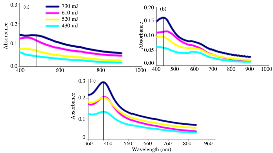
Fig. 5: Absorbance spectrum of nanoparticles of \text{Au}_{50}\text{Ag}_{50} alloy colloidal in SDS solution and at three concentrations 0.25, 0.09, 0.01 molar and at \lambda = 1064 nm, pulse = 100 and in four different energies
