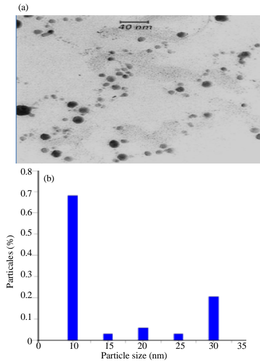
Fig. 4: The TEM image and distribution statistical of nanoparticles of \text{Au}_{50}\text{:Ag}_{50} alloy colloidal in pure water and at using parameters ( \lambda = 1064 \text{ nm} ), ( E = 430 \text{ mJ} ), (pulse = 100) ( f = 6 \text{ Hz} )
