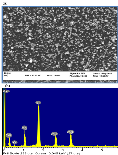
Fig. 2: The SEM images and EDX scheme of nanoparticles of \text{Au}_{50}\text{:Ag}_{50} alloy colloidal in water (DDDW) and at using parameters ( \lambda = 1064 \text{ nm} ), ( E = 610 \text{ mJ} ), (pulse = 100)
