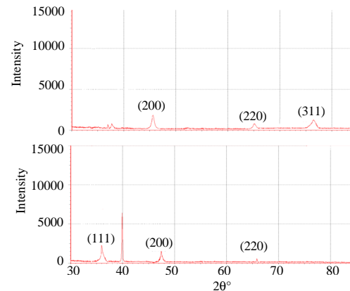
Fig. 8: The X-Ray Diffraction spectra (XRD) of Au:Ag NPS prepared in water, the presence and the absence of the effect (MF) and when ( \lambda = 1064 nm), ( E = 430 mJ) and at the magnetic flux intensity (65 0.1) mT
