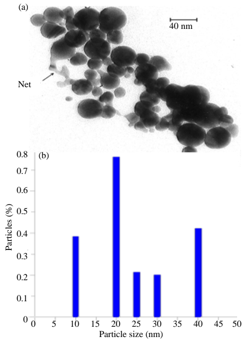
Fig. 3: The TEM image and distribution statistical of nanoparticles of \text{Au}_{50}\text{:Ag}_{50} alloy colloidal in pure water and at using parameters ( \lambda = 1064 \text{ nm} ), ( E = 610 \text{ mJ} ), (pulse = 100) ( f = 6 \text{ Hz} )
