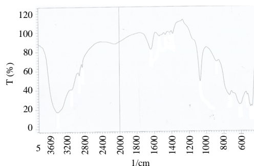
Fig. 2: FT-IR spectrum of electrochemical prepared \text{Al}_2\text{O}_3 -NPs in presence of PVA (1 g/100 mL) as stabilizer and \text{NaNO}_3 (10 g/100 mL) as electrolyte
