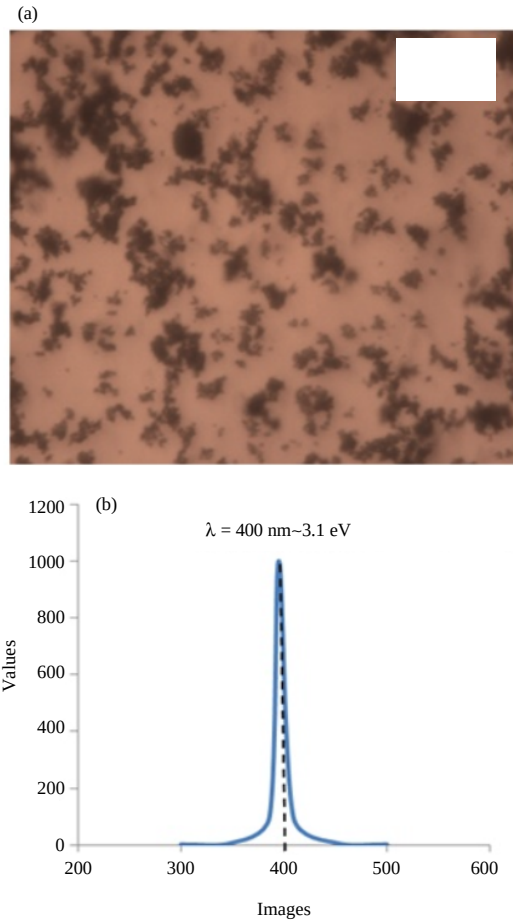
Fig. 7: a) The optical microscope images of ZnO thin films and b) The PL spectra of ZnO thin film
