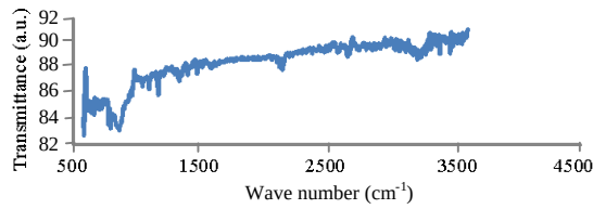
Fig. 4: Observe from the data FTIR spectrum of the pure ZnO
