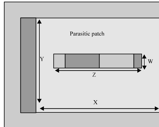
Fig. 2: Geometry of proposed stacked antenna
