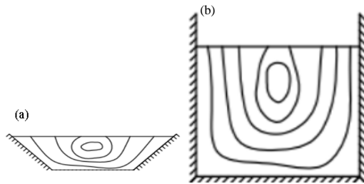
Fig. 2: Velocity distribution in open channel; a) Trapezoidal channel and b) Rectangle channel
