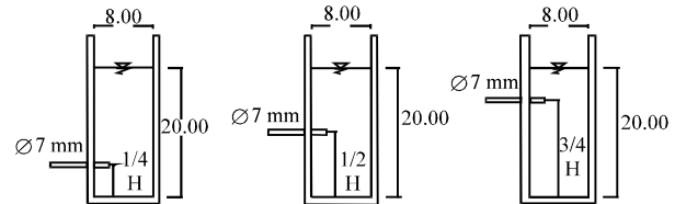
Fig 3: Research flume
