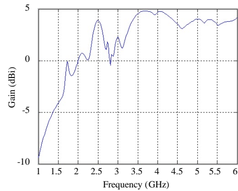
Fig. 4: Gain vs. frequency graph
