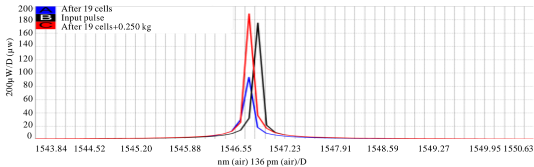
Fig. 9: Thespectrum for pulse laser of source 1 that propagate via. 19 cells: spectrum nm (air) Lin thoriabs OSA, Version 2.55.1299.3162
