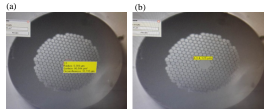
Fig. 5: Images for the cross section for 7 cells under microscope: a) Core diameter and b) The space between two holes ( \Delta )
