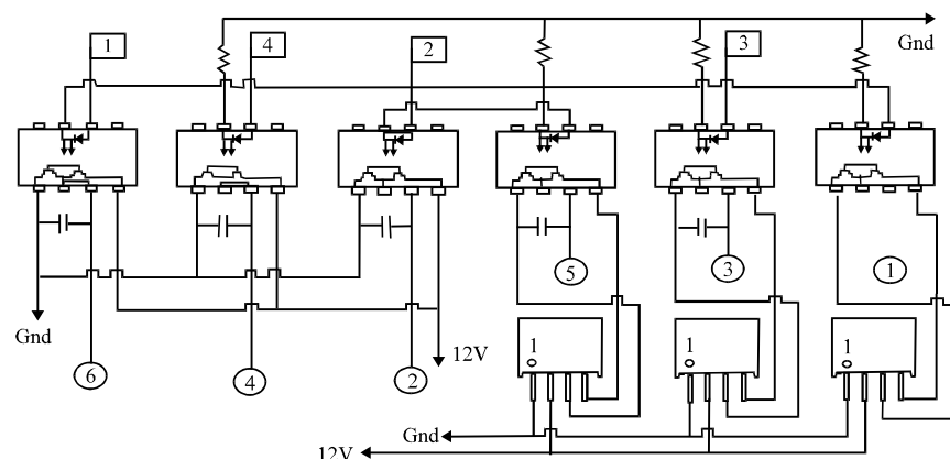
Fig. 10: IGBTs driver circuit
