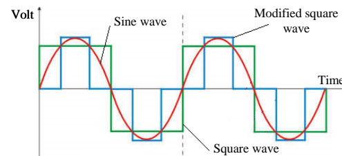
Fig. 3: Sine wave, square wave and modified wave
