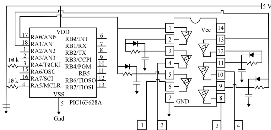
Fig. 9: Micro controller/dead time circuit
