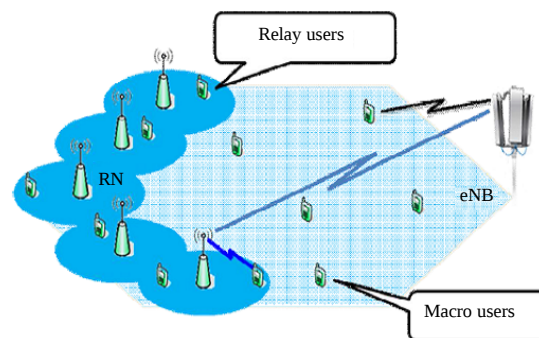
Fig. 1: Transmission links for relays at cell edge on urban macro cell network
