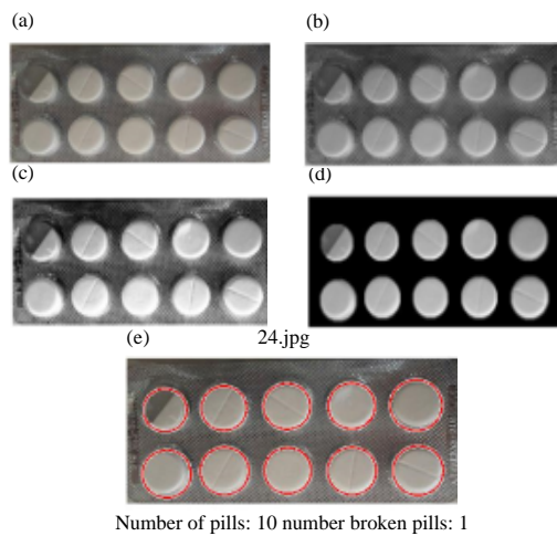
Fig. 4: a) Original image; b) Image after convert to grayscale image; c) Image after histogram equalization; d) Image with pills map overlay and e) Eventual image of the broken tablet
