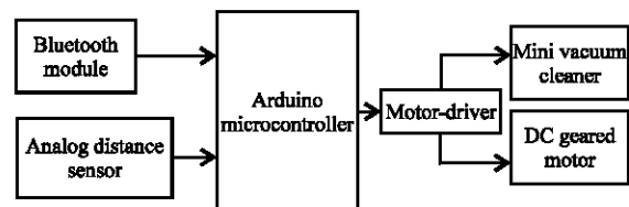
Fig. 1: Block diagram of vacuum cleaner robot
