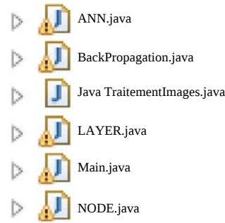
Fig. 8: Classes Java
