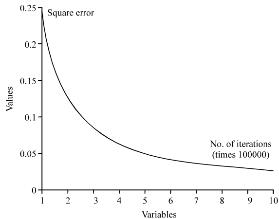
Fig. 9: Convergence graph
