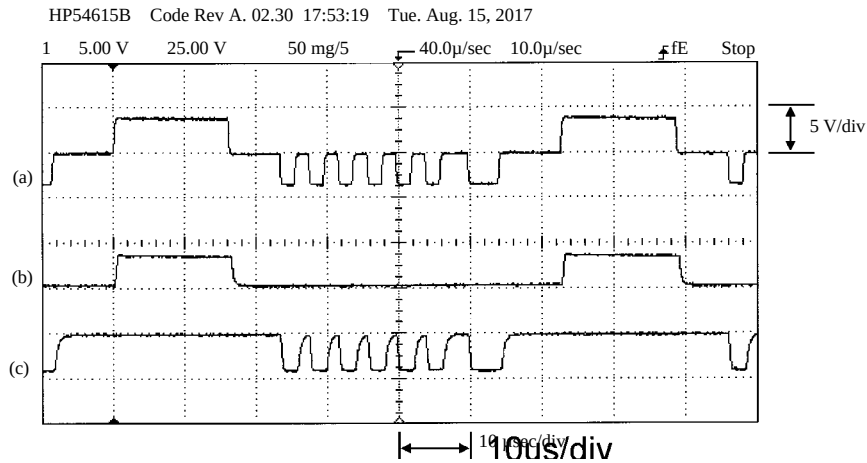
Fig. 7: Waveforms observed in VLC receiver; a) PD voltage; b) Sync pulses and c) Data bits
