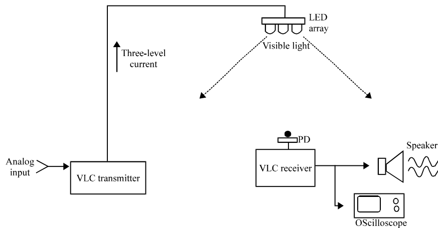
Fig. 5: Experimental setup
