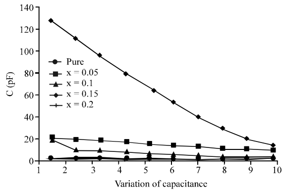
Fig. 4: The variation of capacitance versus reverse bias voltage for (\text{TiO}_2)_{1-x}(\text{CuO})_x/\text{p-Si} heterojunctions at a frequency of 0.5 kHz for different concentrations of CuO
