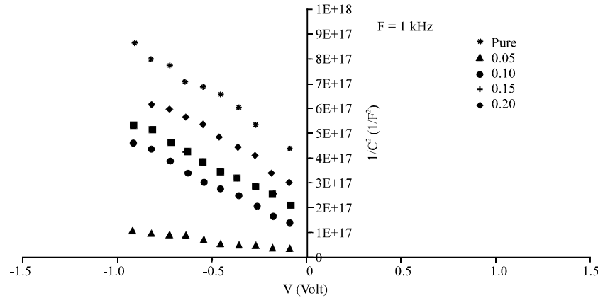
Fig. 7: The inverse of capacitance squared against applied reverse bias voltage for (\text{TiO}_2)_{1-x}(\text{CuO})_x/\text{p-Si} heterojunctions at frequency 1 kHz and different concentrations of CuO
