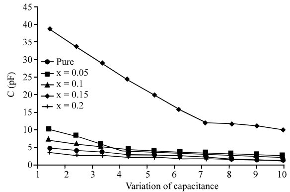
Fig. 5: The variation of capacitance versus reverse bias voltage for (\text{TiO}_2)_{1-x}(\text{CuO})_x/\text{p-Si} heterojunctions at a frequency of 1 KHz for different concentrations of CuO
