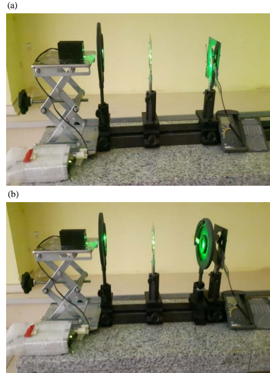
Fig. 1: The construction of a Z-scan with two different designs and the diagram of the possible measured data of the normalized transmittance using them used in this research: a) Closed aperture and b) Open aperture
