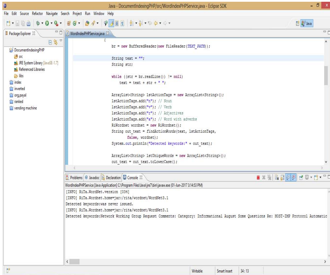
Fig. 4: Keyword extraction
