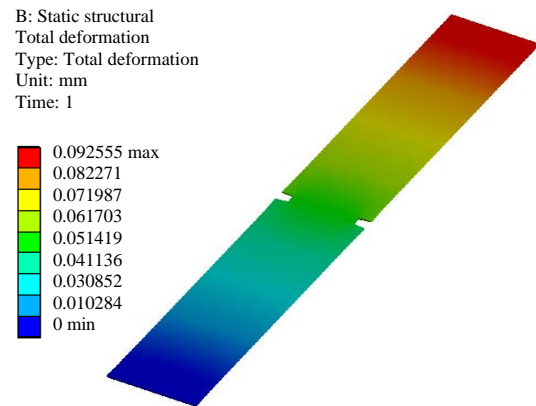
Fig. 7: Total deformation of aluminum notched tensile specimen model
