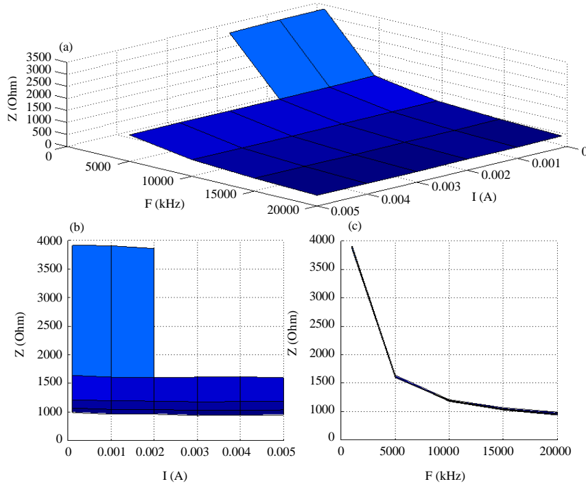
Fig. 9: a) Measurement results of Z between the electrodes E5 and E13 for different values f_i and I_M during exhalation: plot of Z on f_i and I_M ; b) a plot of Z on I_M ; c) plot of Z on f_i
