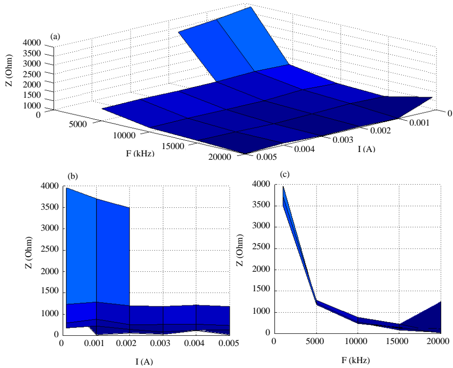
Fig. 8: a) Measurement results of Z between the electrodes E9 and E1 for different values f_i and I_M during exhalation: plot of Z on f_i and I_M ; b) a plot of Z on I_M ; c) plot of Z on f_i
