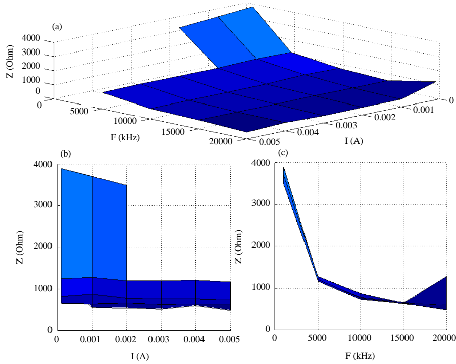
Fig. 7: Measurement results of Z between the electrodes E1 and E9 for different values f_i and I_M during exhalation: a) plot of Z on f_i and I_M ; b) a plot of Z on I_M ; c) plot of Z on f_i
