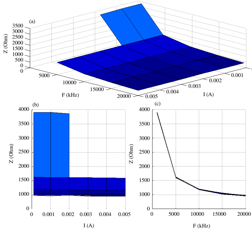
Fig. 10: a) Measurement results of Z between the electrodes E13 and E95 for different values f_i and I_M during inhalation: plot of Z on f_i and I_M ; b) a plot of Z on I_M ; c) plot of Z on f_i
