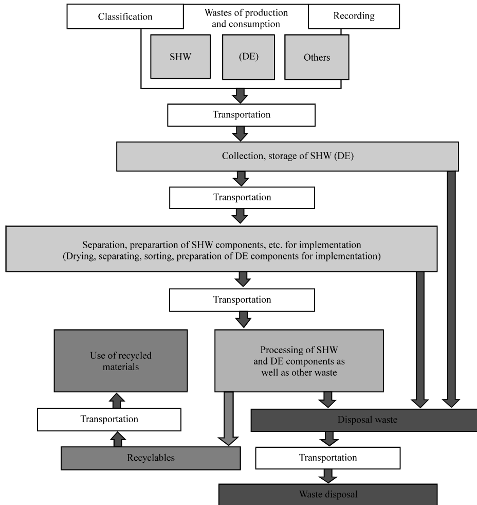
Fig. 2: Waste handling general scheme
