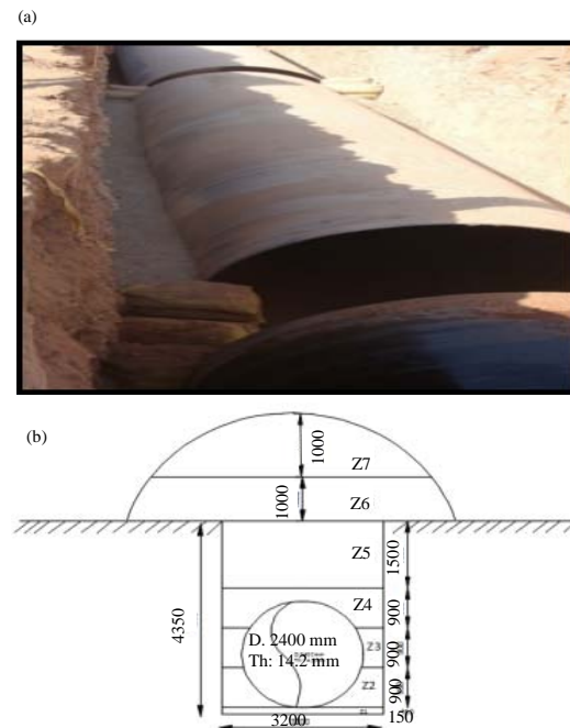
Fig. 5: Type 5 piping
