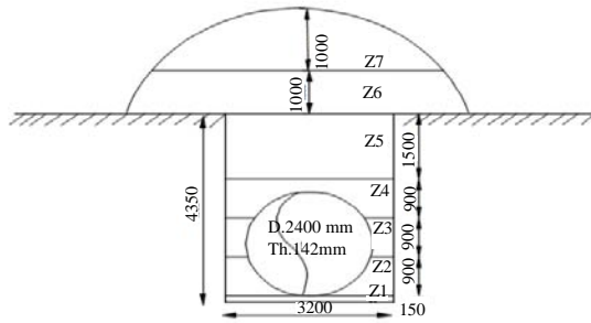
Fig. 3: Type 3 piping
