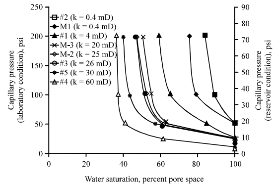
Fig. 3: Measured drainage capillary pressure curves
