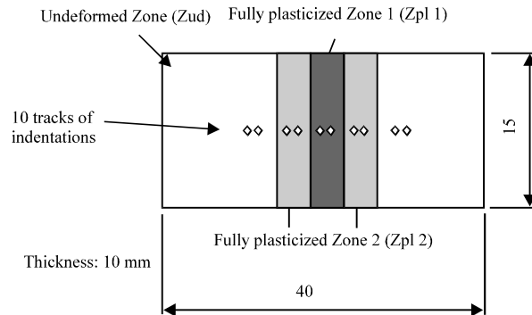
Fig. 4: Indentation locations of micro-Vickers hardness testing on CDFW joint
