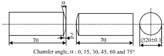
Fig. 1: Geometry of CDFW specimen (dimensions in mm). Left side is rotated part and the right side is stationary part that subjected with compression force
