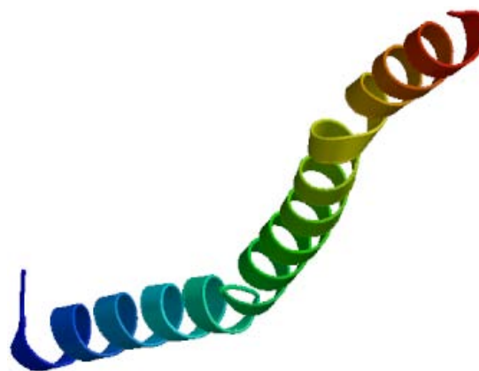
Fig. 2: 3D structure of VhhP2
