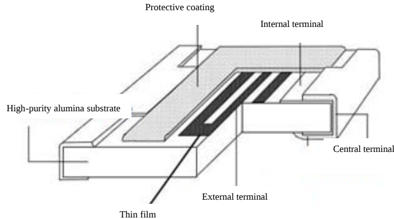
Fig. 2: Structure of SMD resistances
