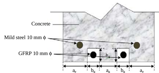
Fig. 2: Groove details; b_g and h_g = 20 mm a_g = 30 mm a_e = 40 mm
