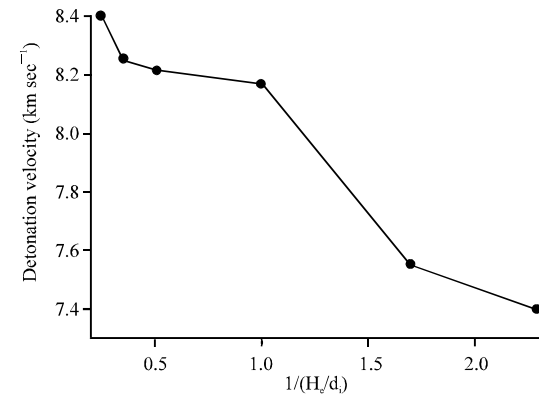
Fig. 2: Detonation velocity as a function of 1/(H_e/d_i) ( D_u )
