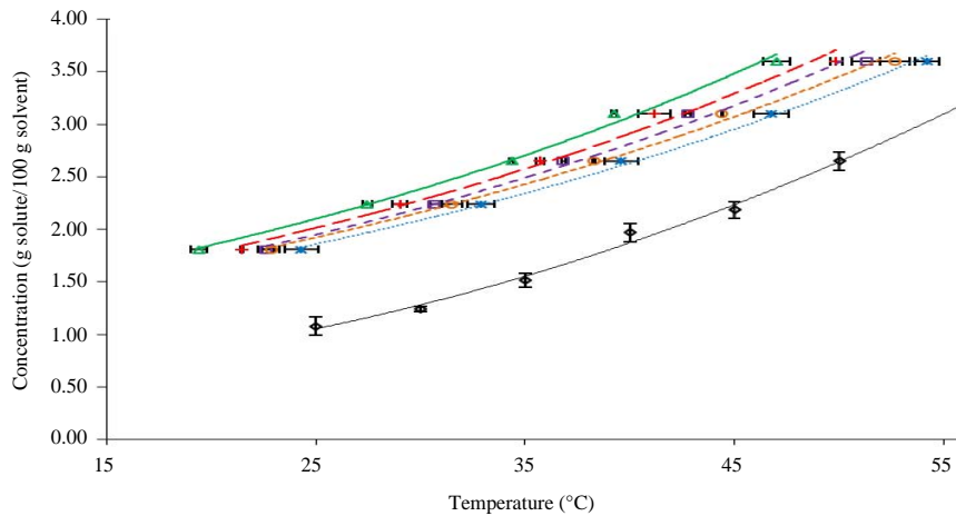
Fig. 7: Solubility (Abdul et al. , 2013) ( \diamond ) and metastable zone width data of mefenamic acid in ethyl acetate for five different cooling rates: * = 0.2^{\circ}\text{C}/\text{min} ; \Delta = 0.5^{\circ}\text{C}/\text{min} ; \Delta = 1.0^{\circ}\text{C}/\text{min} ; + = 2.5^{\circ}\text{C}/\text{min} ; D = 5^{\circ}\text{C}/\text{min} . The solid and dotted lines either in black, blue, brown, purple, red or green colors are the best fit to represent the solubility and metastable zone width data with R^2 values above 0.95
