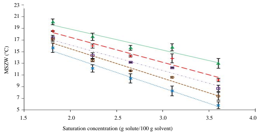
Fig. 8: The dependency of MSZW on saturation concentration measured at different cooling rates: * = 0.2^{\circ}\text{C}/\text{min} ; o = 0.5^{\circ}\text{C}/\text{min} ; \Delta = 1.0^{\circ}\text{C}/\text{min} ; + = 2.5^{\circ}\text{C}/\text{min} ; D = 5^{\circ}\text{C}/\text{min} . The solid or dotted lines which are either in blue, brown, purple, red or green colors are the best fit to represent the trend. The R^2 values are above 0.95
