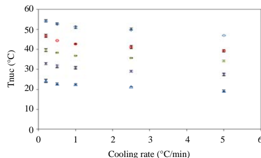
Fig. 6: Nucleation temperature, at different cooling rates for mefenamic acid solutions saturated at 40°C (Δ) 45°C (x), 50°C (*), 55°C (o), and 60°C (◇) in 500 mL
