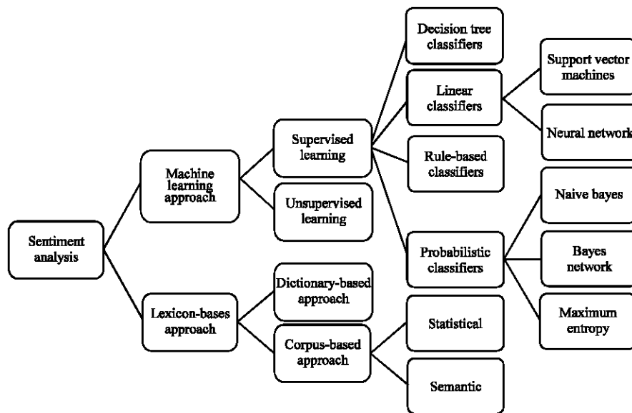
Fig. 1: Sentiment classification techniques used in sentiment analysis (Medhat et al. , 2014)
